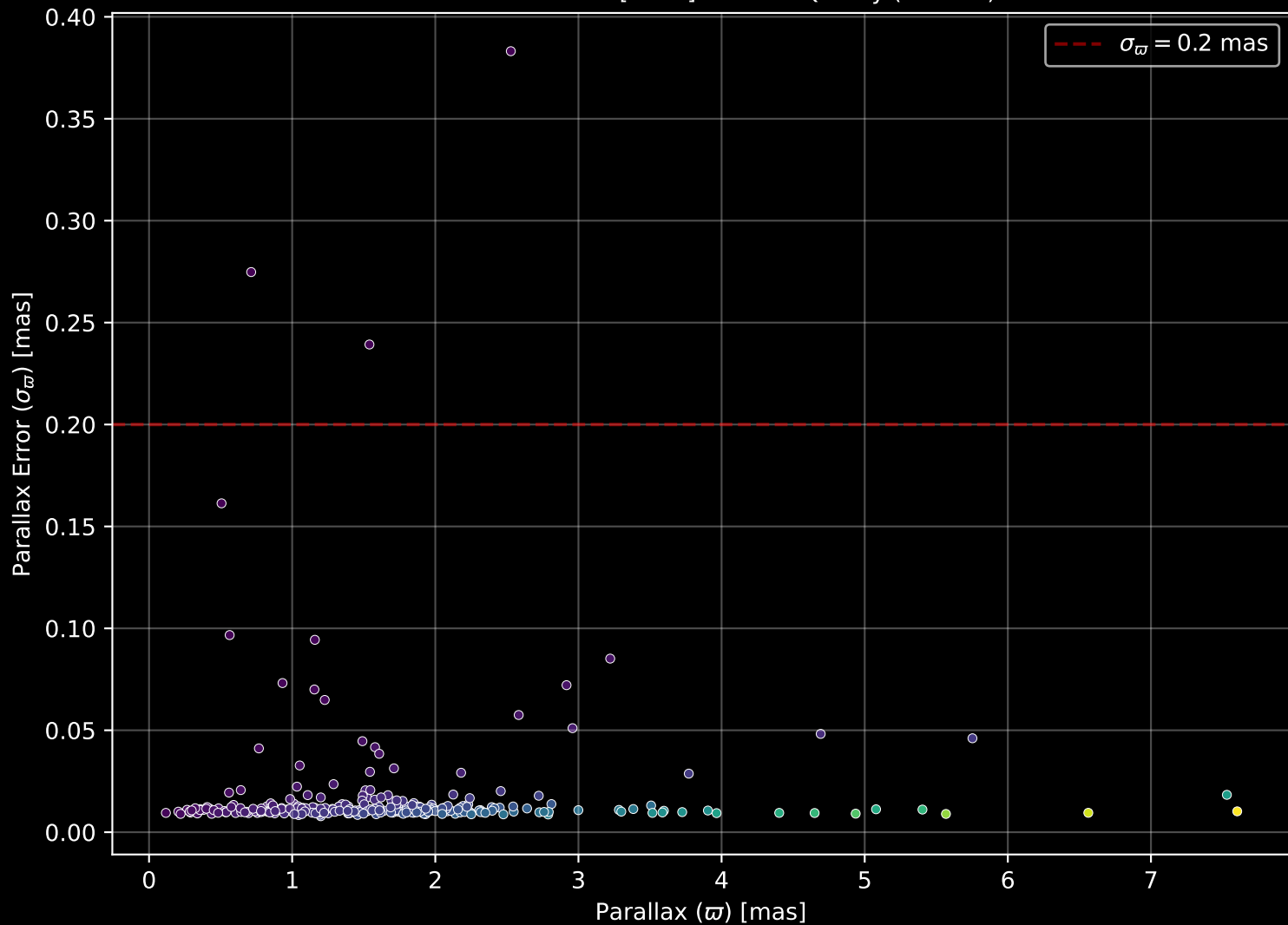
GALAH DR4 Field: [1111] Parallax Quality (n= 298)
