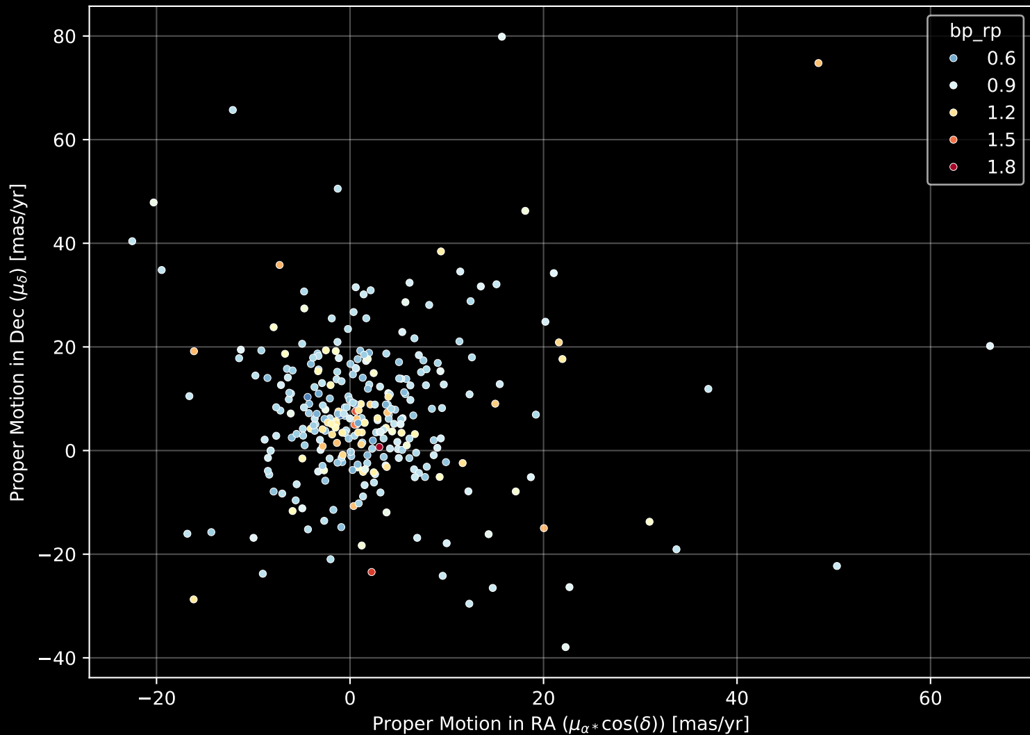
GALAH DR4 Field: [1111] Proper Motion Diagram (n= 298)
