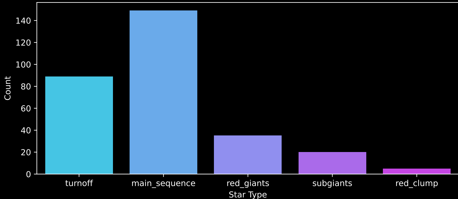
GALAH DR4 Field: [1111] Count plot of Star Type
