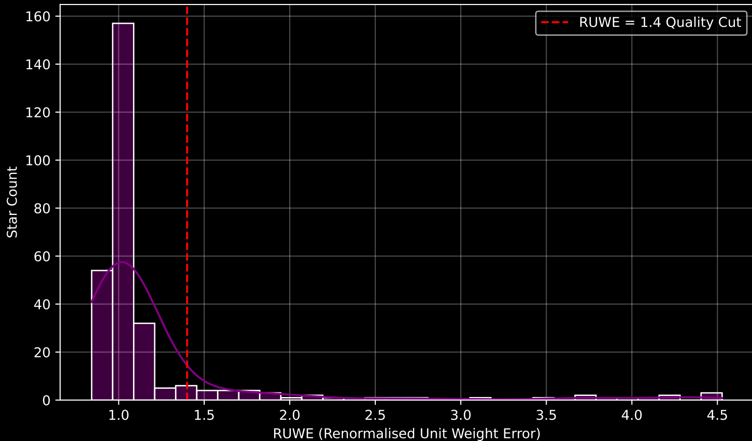
GALAH DR4 Field [1111] RUWE Distribution (n= 287)
